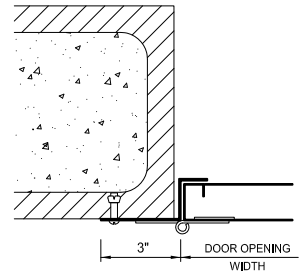
JAMB DETAIL CONCRETE BLOCK
